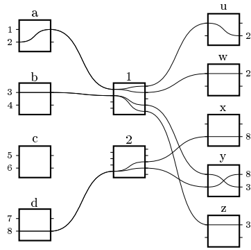
(a) Clos 2-cast network C(2, 4, 2, 2, 5) with 3 connecting paths.
