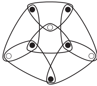
(a) Hypergraph H . Black vertices belong to out-partition, white vertices belong to in-partition, \Delta(H) = 3 .
