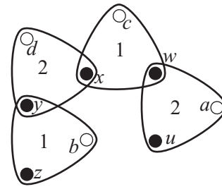
(d) Hypergraph corresponding to the Clos network (c) and its coloring.
