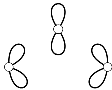
(c) Graph induced by set V_i of H , H(V_i) . \Delta_i = 2 .
