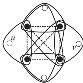
Figure 6: Gadget for complete graphs. The dashed lines mark underlying K_4 .
