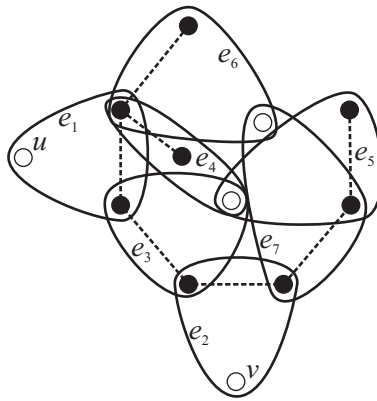
Figure 5: Gadget for forest. The dashed lines mark an underlying tree.
