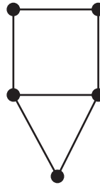
(d) Graph induced by set V_o of H , H(V_o) . \Delta_o = 3 .
