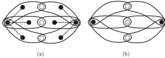
Figure 8: Illustration for the proof of Theorem 2. (a) Example of a bipartite hypergraph. (b) Bipartite multigraph corresponding to (a).
