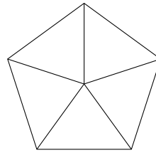
(b) Line graph L(H) , \Delta(L(H)) = 5 .
