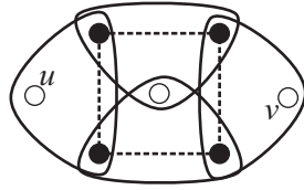
Figure 4: Gadget for cycle. The dashed lines mark underlying cycle C_4 .
