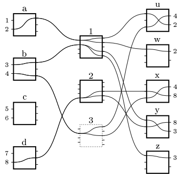
(e) Clos network (a) with one additional call (from b to u and x) that cannot be rerouted and needs the 3rd middle switch.
