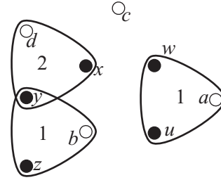
(b) Hypergraph corresponding to the Clos network (a) (vertices from V_0 are black and from V_i are white) and its coloring (numbers inside hyperedges).
