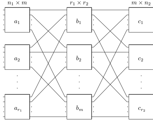
Figure 1: Example of Clos network C(n_1, r_1, m, n_2, r_2) .
