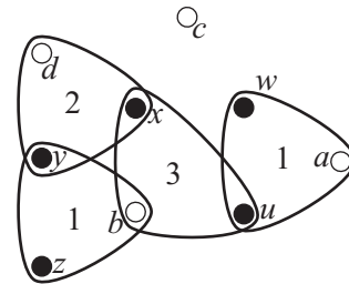
(f) Hypergraph corresponding to the Clos network (e) and its coloring.
