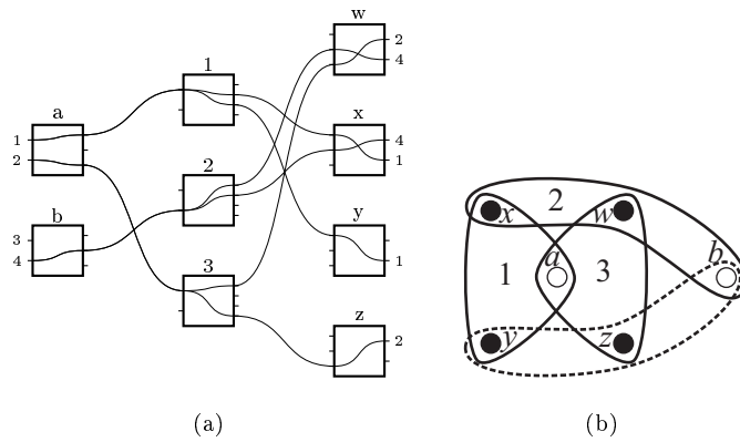
Figure 9: (a) Clos network C(2, 2, 3, 2, 4) with 3 connecting paths. A new call (from b to y and z ) would be blocked; (b) Corresponding hypergraph. The new call is marked with a dashed cycle.
