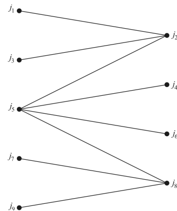
Fig. 1. Example of incompatibility graph.
