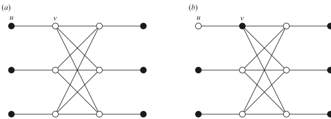
Fig. 3. K_{3,3} and its neighborhood (vertices in black belong to I_1 ): (a) before interchange; (b) after interchange.
