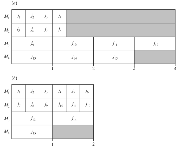
Fig. 7. Gantt chart of a schedule for Algorithm 3 with graph of Fig. 4 when s_1 = s_2 = 3s_3 = 3s_4 : (a) worst-case schedule; (b) optimal schedule.
