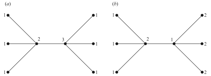
Fig. 6. Graph G with two colorings: (a) of type [6, 1, 1, 0] ; (b) of type [4, 4, 0, 0] .
