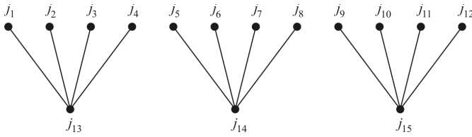
Fig. 4. Example of incompatibility graph G = 3K_{1,4} .
