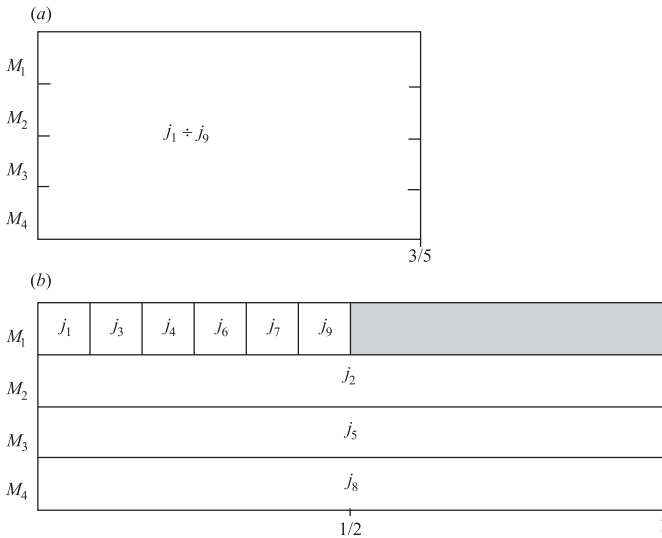
Fig. 2. Gantt chart of a schedule for graph of Fig. 1 when s_1 = 12, s_2 = s_3 = s_4 = 1 : (a) ideal; (b) optimal.
